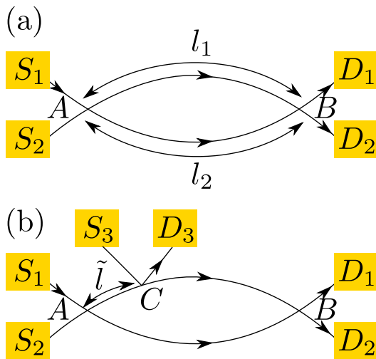
FIG. 1. Illustration of the Mach-Zehnder interferometers (MZIs) under study. Chiral channels are represented by full lines leading from the sources ( S_1 — biased and S_2 — grounded) to the drains ( D_1 and D_2 ). Inter-edge tunneling takes place at intersection points. (a) A standard MZI with arms 1 and 2 of lengths l_1 and l_2 , respectively. (b) The dangling end at C (leading to D_3 ) serves as an absorber replacing the “lousy” bomb.
