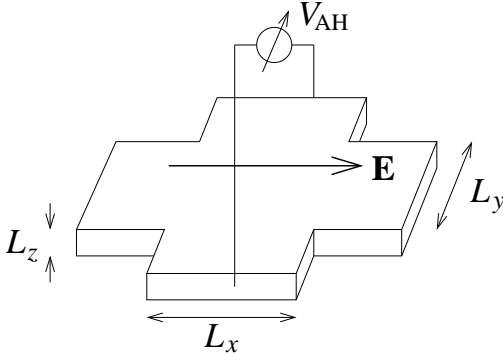
FIG. 1: Geometry of the relevant section of the Hall bar.
