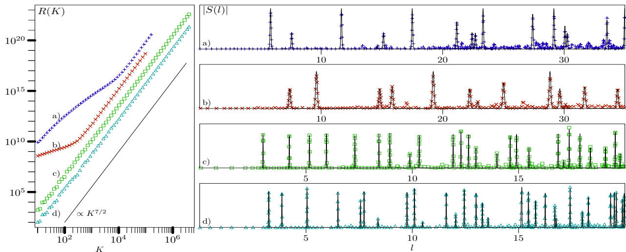
FIG. 1: Numerical checks of the fluctuating parts of trace formulae for the two ellipsoids ( a) and b), see text) and the two tori ( c) and d), see text). left : Double logarithmic plot of the integrated squared fluctuations (20) (arbitrary scale), the full line has slope 7/2 . Right : Length spectra of the nodal counting functions (21). The full line is obtained from the trace formulae (19) and (7) and the points represent the numerical data.
