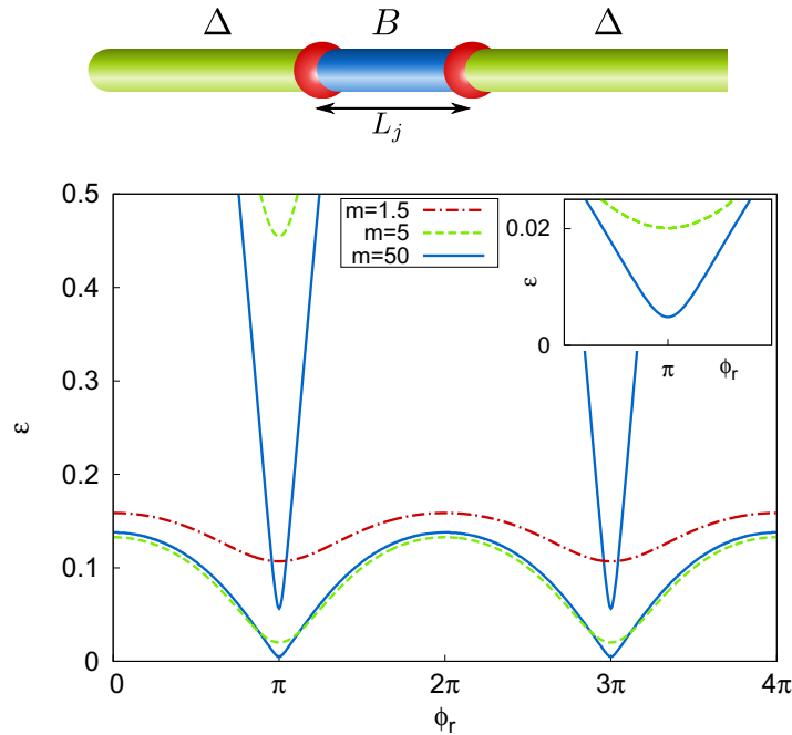
Figure 5. Low-energy spectrum of a \Delta - B - \Delta junction as function of \phi_r for different masses m (and hence spin-orbit energies \epsilon_{SO} = mu^2 ). As indicated by table 1, the spectrum approaches 4\pi periodicity for \epsilon_{SO} \rightarrow \infty . For strong spin-orbit coupling, Andreev bound states appear. Their energy has a phase dependence \epsilon_A \sim \Delta \cos(\phi/2) . Inset: close-up near \phi = \pi showing the avoided crossing at \epsilon = 0 . Parameters: B_{l/r} = \Delta_m = 1 , \Delta_{l/r} = B_m = 2 , u = 1 , \mu_{l/m/r} = 0 , L_j = 2 and \theta_{l/m/r} = \phi_{l/m} = 0 .
