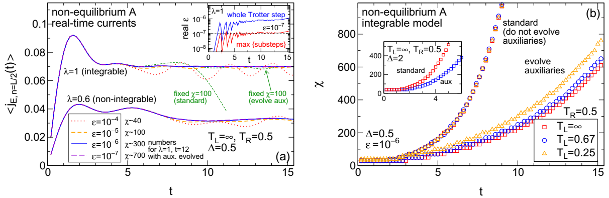
Figure 3. DMRG time evolution of an XXZ chain of length L = 200 featuring an initial sharp temperature gradient T_L \neq T_R . The system is gapless for z -anisotropies |\Delta| \leq 1 and gapped otherwise; it becomes non-integrable in presence of a finite dimerization \lambda < 1 . Note that for \Delta = 0.5 and \lambda = 1 asymptotic low-temperature behavior described by a field theory [77] sets in for T \lesssim 0.2 . (a) Energy current at the interface. Choosing a discarded weight control parameter around \epsilon \sim 10^{-6} at a Trotter stepsize of \Delta t = 0.2 is sufficient to accurately obtain its steady-state value. Inset: the actual discarded weights during a whole Trotter step and during one substep for \Delta\chi = 20 . The difference to \epsilon is explained in the main text. (b) Evolution of the dimension of the corresponding matrix product state. If the auxiliary degrees of freedom which purify the thermal density matrix are time-evolved with the physical Hamiltonian but reversed time (which is an exact modification to the standard algorithm), the build-up of entanglement is reduced. The computational cost of a singular value decomposition (which dominates the DMRG algorithm) scales as \chi^3 .
