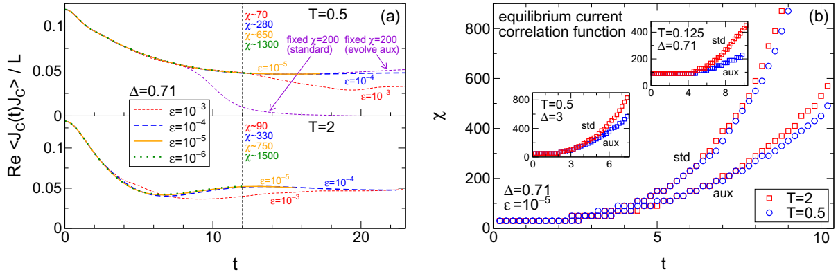
Figure 5. (a) DMRG calculation of the global charge current correlation function \langle J_C(t)J_C \rangle of the integrable XXZ chain (length L = 100 ) in thermal equilibrium. The calculation is stopped once \chi reaches values around \chi \sim 1500 ; the numbers in the plot denote \chi at time t = 12 for the different discarded weights (the auxiliaries are time-evolved). (b) Evolution of the corresponding MPS dimension for different anisotropies \Delta = 0.71 (gapless) and 3 (gapped).
