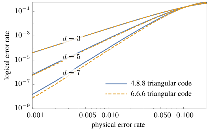
FIG. 24. Logical error rate of the first three 4.8.8 and 6.6.6 triangular color codes. Even though the codes have the same code distance and error threshold, 4.8.8 color codes have a higher logical error rate, but require fewer physical qubits per logical qubit.
