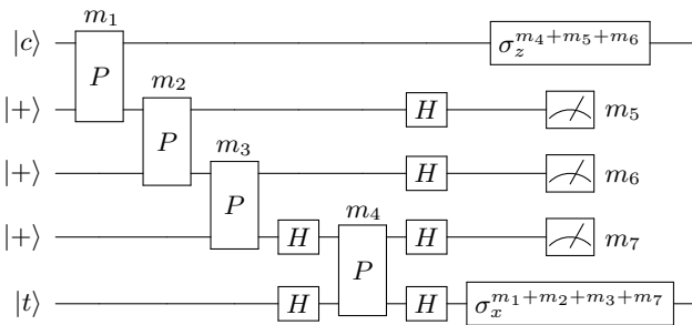
FIG. 22. Quantum circuit corresponding to the constant time overhead CNOT gate in Fig. 10.
