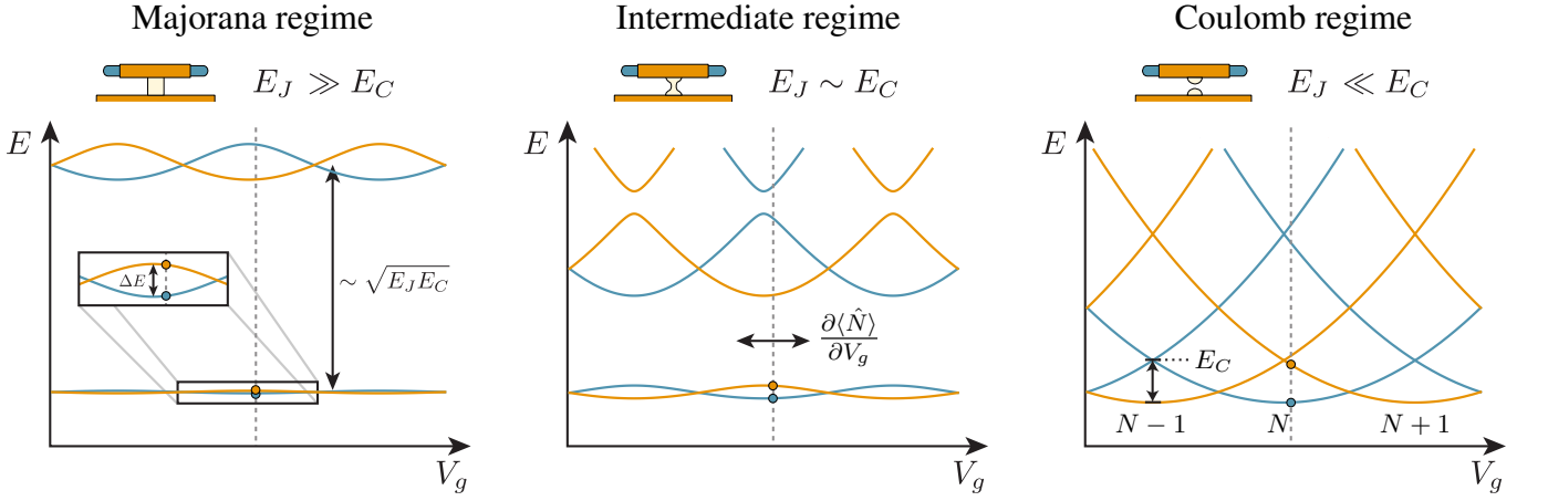
FIG. 15. Parity-to-charge conversion in the Majorana Cooper pair box, as described in Ref. [32], and energy levels of the Majorana Cooper pair box H_C + H_J as a function of gate voltage V_g and for different ratios E_J/E_C . In the Majorana regime E_J \gg E_C , charging energy is negligible and the spectrum is insensitive to V_g . The ground state is given by nearly-degenerate states of opposite parity (blue and orange), where the maximum separation \Delta E vanishes exponentially in E_J/E_C , whereas the distance to the first excited states increases with \sqrt{E_J E_C} . As E_J is decreased by decreasing the coupling to the bulk superconductor, the ground state degeneracy is lifted in the intermediate regime. Here, varying the gate voltage distinguishes the parity states through their differential capacitance C = \partial\langle\hat{N}\rangle/\partial V_g , which is larger for the orange parity than for the blue parity. Finally, in the Coulomb regime E_J \ll E_C , the spectrum is given by parabolas with well-defined charge number N . If V_g is tuned to a minimum of a charge parabola, the two lowest-energy parity states are separated by E_C , which can be used to impose a certain parity on the island. The intermediate regime can also be understood from the emergence of avoided crossings between charge states of equal parity as E_J is increased.
