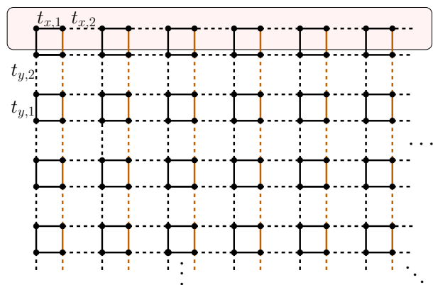
FIG. 2. Tight-binding model for a second order topological insulator on a square lattice. Solid and dashed lines in the x and y directions denote alternating nearest neighbor hoppings t_{x,1} , t_{x,2} and t_{y,1} , t_{y,2} . The hopping amplitudes for the bonds colored in brown include a relative minus sign. The effective Hamiltonian of the highlighted boundary parallel to the x -direction is topologically equivalent to an SSH model.
