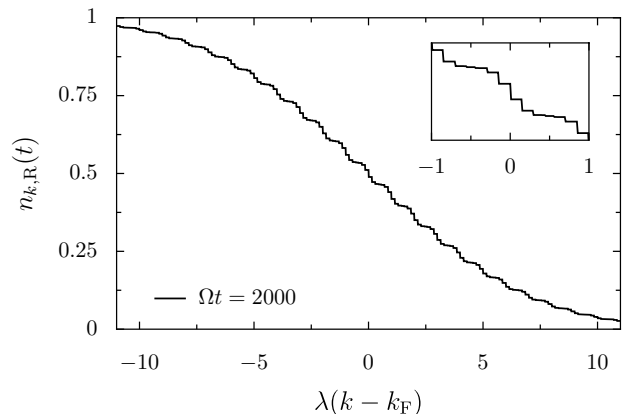
Fig. 3: Momentum distribution for right movers n_{k,R}(t) in the long-time regime (see eq. (17)) as a function of momentum k . The parameters are the same as in fig. 2(a). The inset presents the momentum distribution at a finer wave number scale close to the Fermi level.
