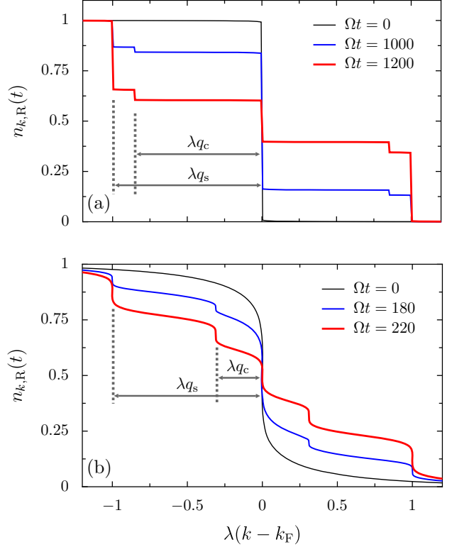
Fig. 2: (Colour on-line) Fermionic momentum distribution for right movers n_{k,R}(t) in the short-time regime (see eq. (15)) as a function of momentum k , scaled by the screening length \lambda . In the figure, T = 0 , \gamma = 0.1 and \lambda q_s = 1 . (a) Case of contact s -wave scattering interaction, with V_0^+ / v_F = 0.5 and V_0^|| = V_{2k_F}^|| = 0 , such that \lambda q_c = \lambda q_s v_s / v_c \simeq 0.85 . (b) Case of finite-range interactions, with V_0^|| / v_F = V_0^+ / v_F = 10 and V_{2k_F}^|| / v_F = 2 , such that \lambda q_c = \lambda q_s v_s / v_c \simeq 0.31 . Thicker lines correspond to larger times t .
