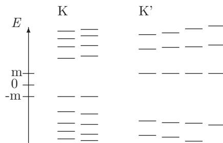
Fig. 2: Same sketch as in fig. 1 but now including a real magnetic field with \Phi_{EM} = -3.2\phi_0 . (The horizontal position only used to guide the eye.) The quasi-Landau levels are broadened by the ripples, except the Landau level of the threshold modes. However, with \Phi_{rip} = 1.1\phi_0 and therefore \Phi^K = \Phi_{EM} + \Phi_{rip} = -2.1\phi_0 and \Phi^{K'} = \Phi_{EM} - \Phi_{rip} = -4.3\phi_0 the threefold degeneracy of the threshold modes at E = -m ( E = +m ) of valley K (K’) becomes twofold (fourfold). The rest of the spectrum is in each valley symmetric about E = 0 due to supersymmetry.
