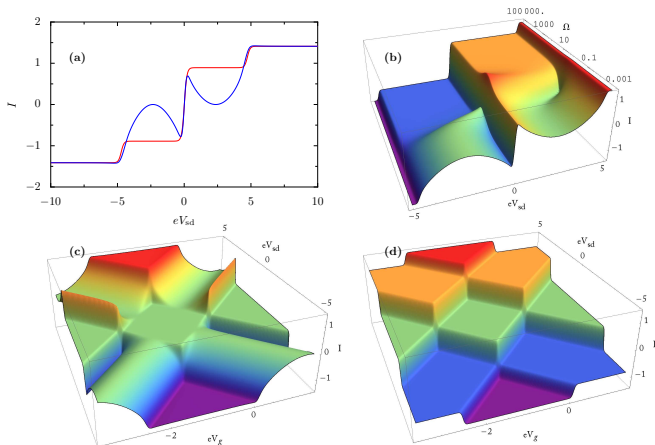
FIG. 1: (Color online) Numerical evaluation of the stationary current Eq. (9) through an interacting two-level Anderson model, t_{L\uparrow} = t_{R\downarrow} = 1 , t_{L\downarrow} = t_{R\uparrow} = 1.5 , U = 2.35 , k_B T = 0.02 . The tunnel amplitudes t_{\alpha\sigma} and the splitting \Omega are measured in units of \frac{2\pi}{\hbar}\nu_0 . Fig. (a) illustrates the difference between the description by the degenerate master equation, Eqs. (7, 8), (blue) and the \Omega = 0 rate equation, which is obtained from the master equation by setting \rho_{\uparrow\downarrow} = 0 (red). Both models are evaluated at eV_g = 0 in order to highlight the quantitative as well as qualitative discrepancy. In Figs. (c) and (d), we show a full scan of the (eV_g, eV_{sd}) -plane for both equations, illustrating the fundamental difference of the dynamics due to the two equations in the parameter space. While the rate-equation result is the familiar sequence of steps in the stationary current, the master-equation result shows a strong current suppression for voltages below the double-charging threshold. Using the master equation in the singular-coupling limit as it is derived in the text, we interpolate the two different curves of Fig. (a) by letting \Omega \rightarrow \infty in Fig. (b).
