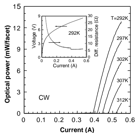
Fig. 2. CW optical power from a single laser facet as a function of drive current for various heat sink temperatures. The laser is 0.75 mm long and 12 μm wide. The power was measured with near-unity collection efficiency and a calibrated thermopile detector. (Inset) Electrical transport characteristics of the laser at 292 K: bias voltage as a function of injection current and differential resistance deduced from the V - I curve.
